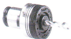
絲攻接頭 (Tapping Adapter) 扭力保護型 (with safety clutch)
